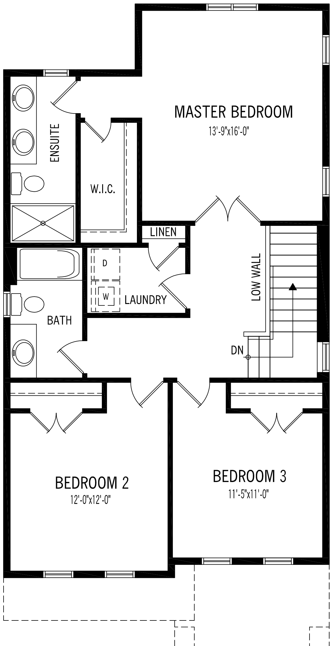
SECOND FLOOR PLAN 1017 SQ.FT.
