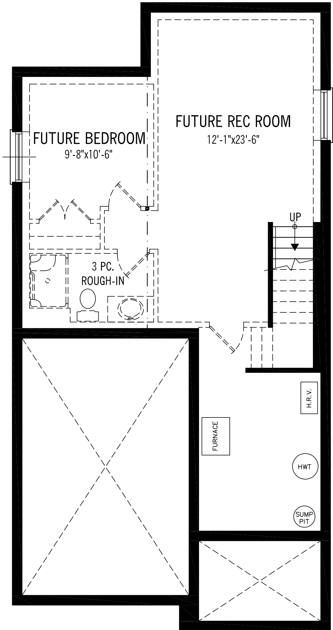
BASEMENT PLAN
