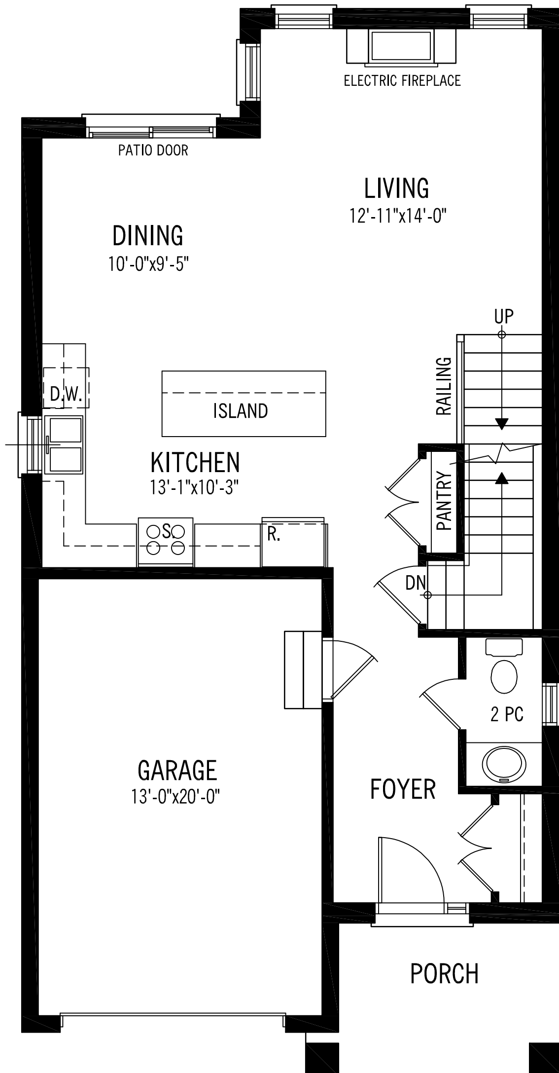
MAIN FLOOR PLAN 769 SQ.FT.
